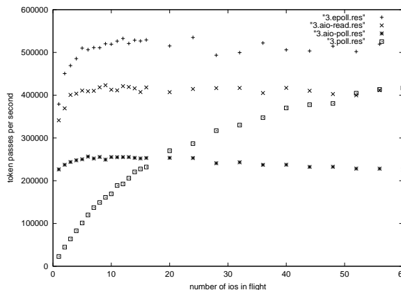
Figure 5: thruput while increasing in flight ios
